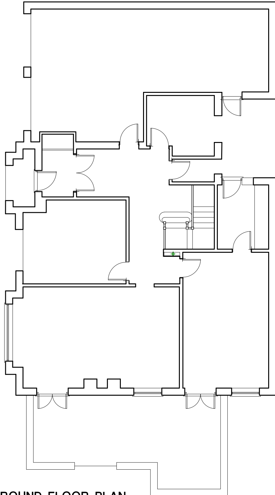
GROUND FLOOR PLAN 110.54 sq mtrs gross internal
