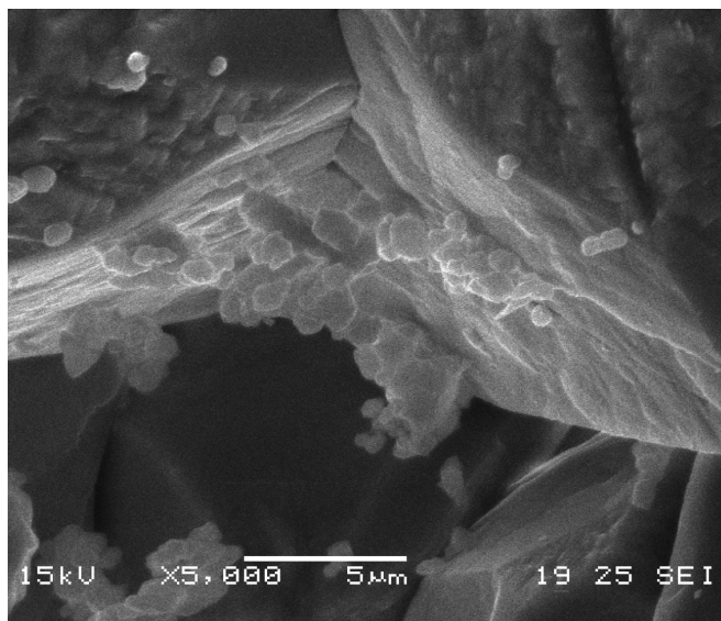
Figure 8 Scanning Electron Microscope (SEM) image showing nanolime particles deposited on the internal pore walls of Bath stone (Magnification x5000).
