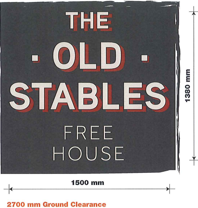
ITEM 04B (Qty 1) Signwriting to planked wall area. Scale 1:20
