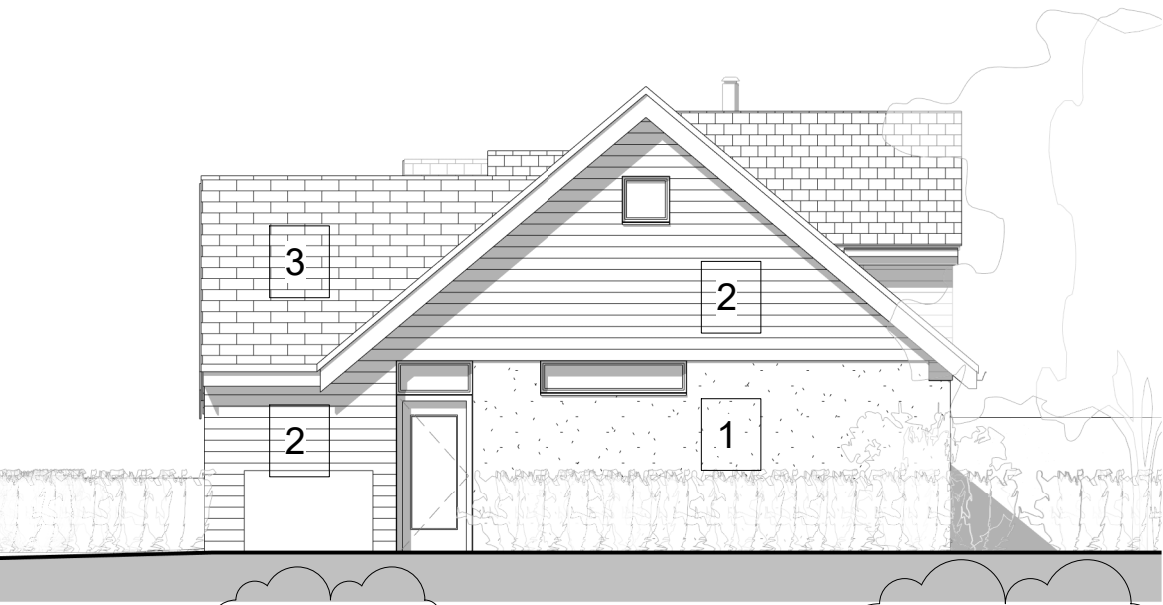
North Elevation 1 : 100
