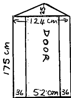
SHED FRONT
