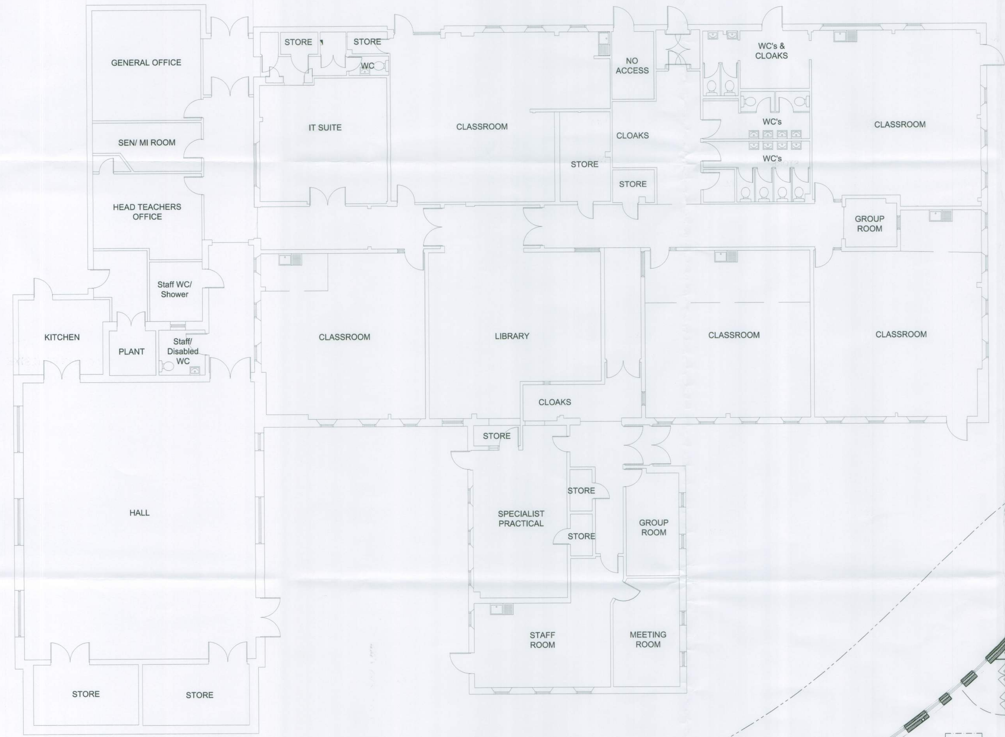
EXISTING BUILDING PLAN
