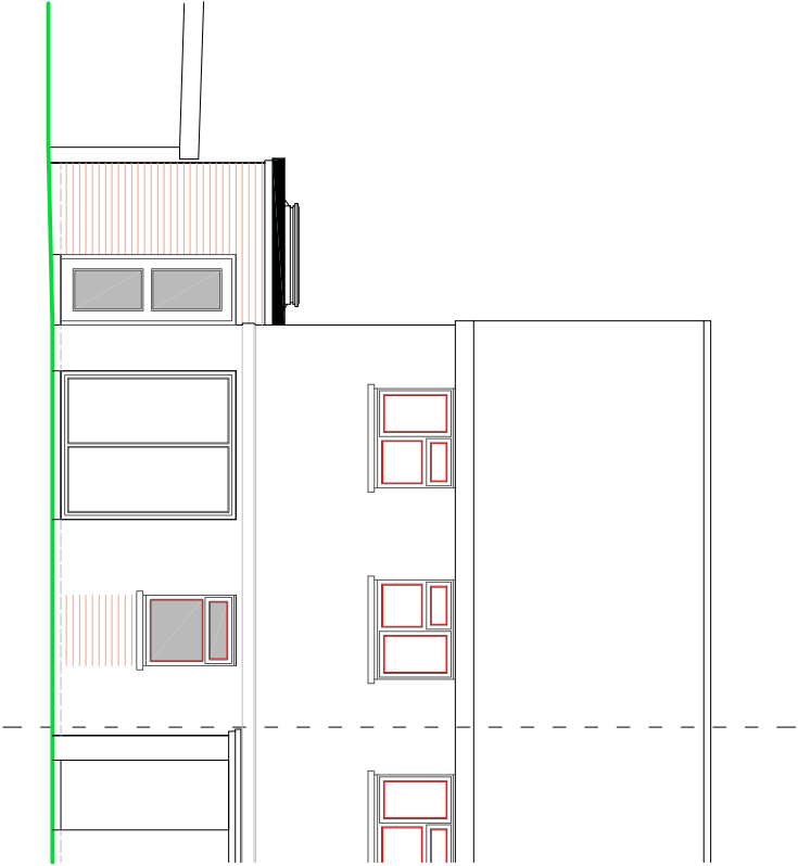
REAR ELEVATION
