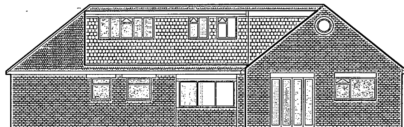
Rear Elevation (East Elevation)
