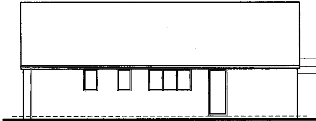
EXISTING SIDE SOUTH EAST FACING ELEVATION
