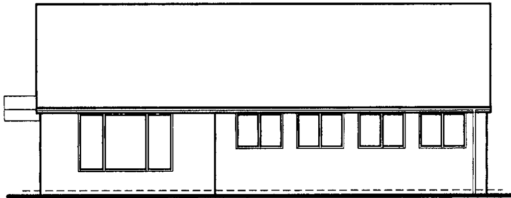
EXISTING SIDE NORTH WEST FACING ELEVATION
