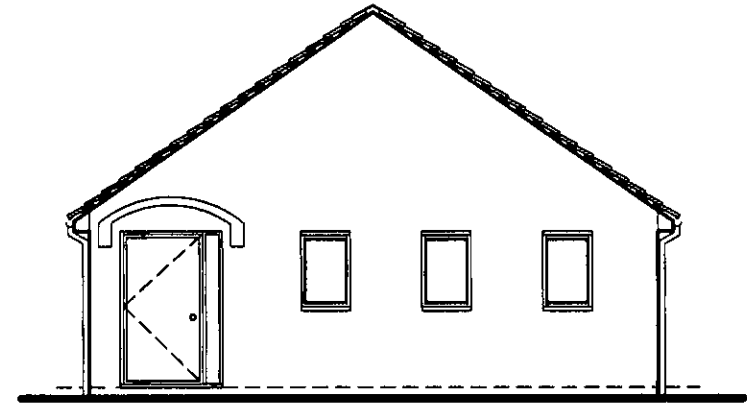
EXISTING FRONT NORTH EAST FACING ELEVATION
