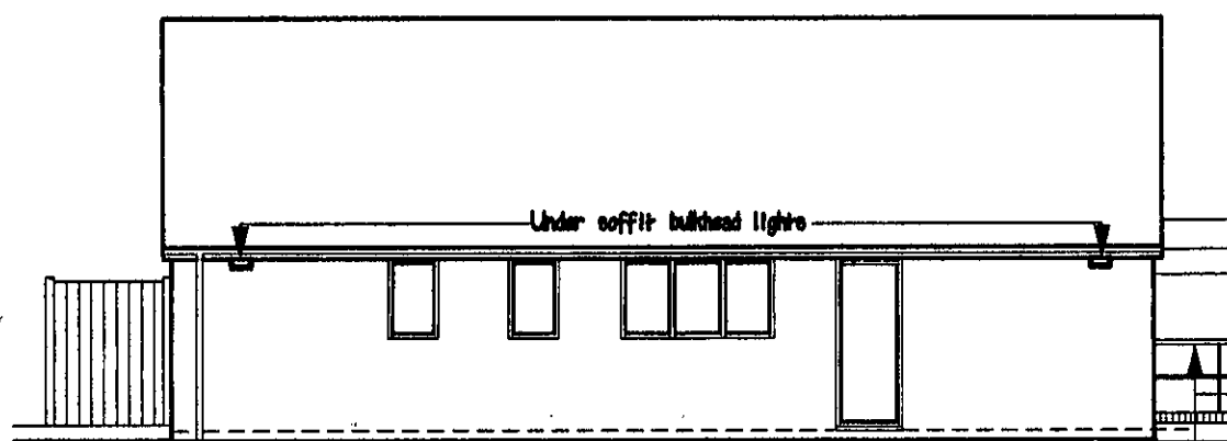
PROPOSED SIDE SOUTH EAST FACING ELEVATION
