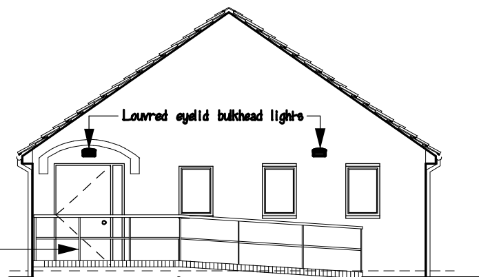
PROPOSED FRONT NORTH EAST FACING ELEVATION
