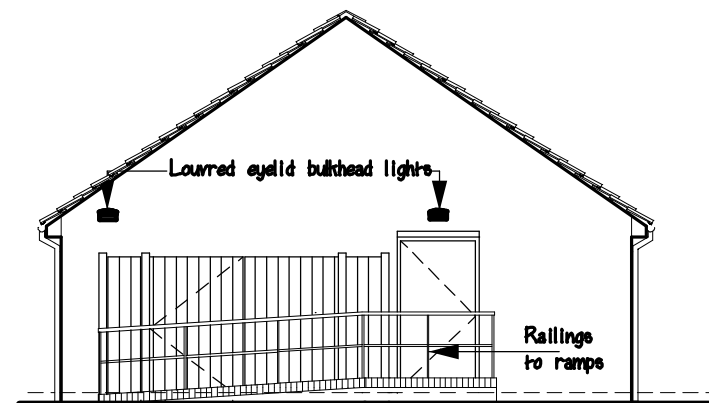
PROPOSED REAR SOUTH WEST FACING ELEVATION
