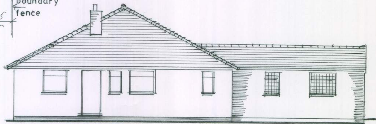
EXISTING EAST VIEW 1:100
