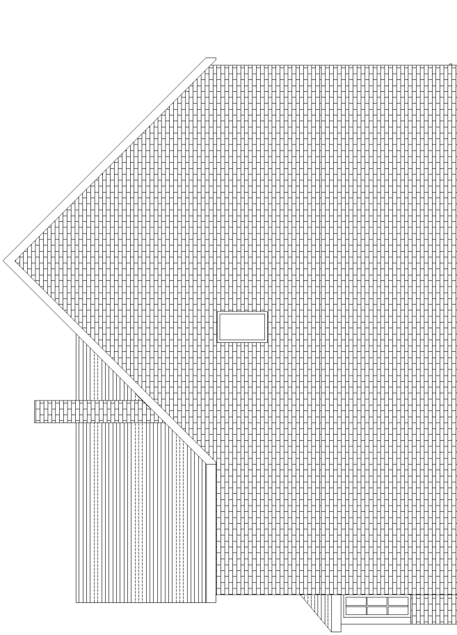
Existing SW Elevation 1 : 100
