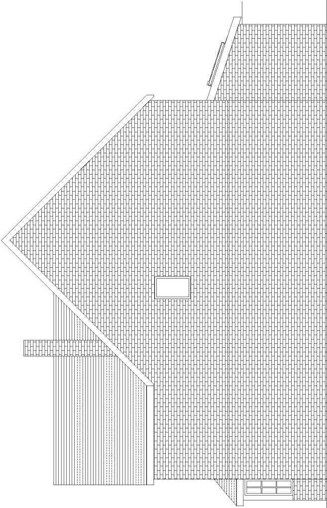
Proposed SW Elevation 1 : 100
