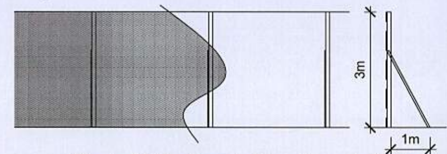
Typical Windbreak Elevations 1:100
