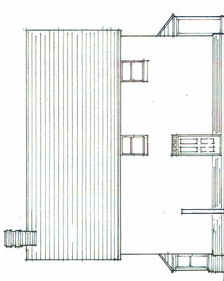
REAR ELEVATION
