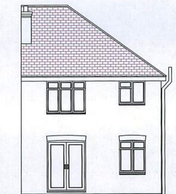
Rear Elevation
