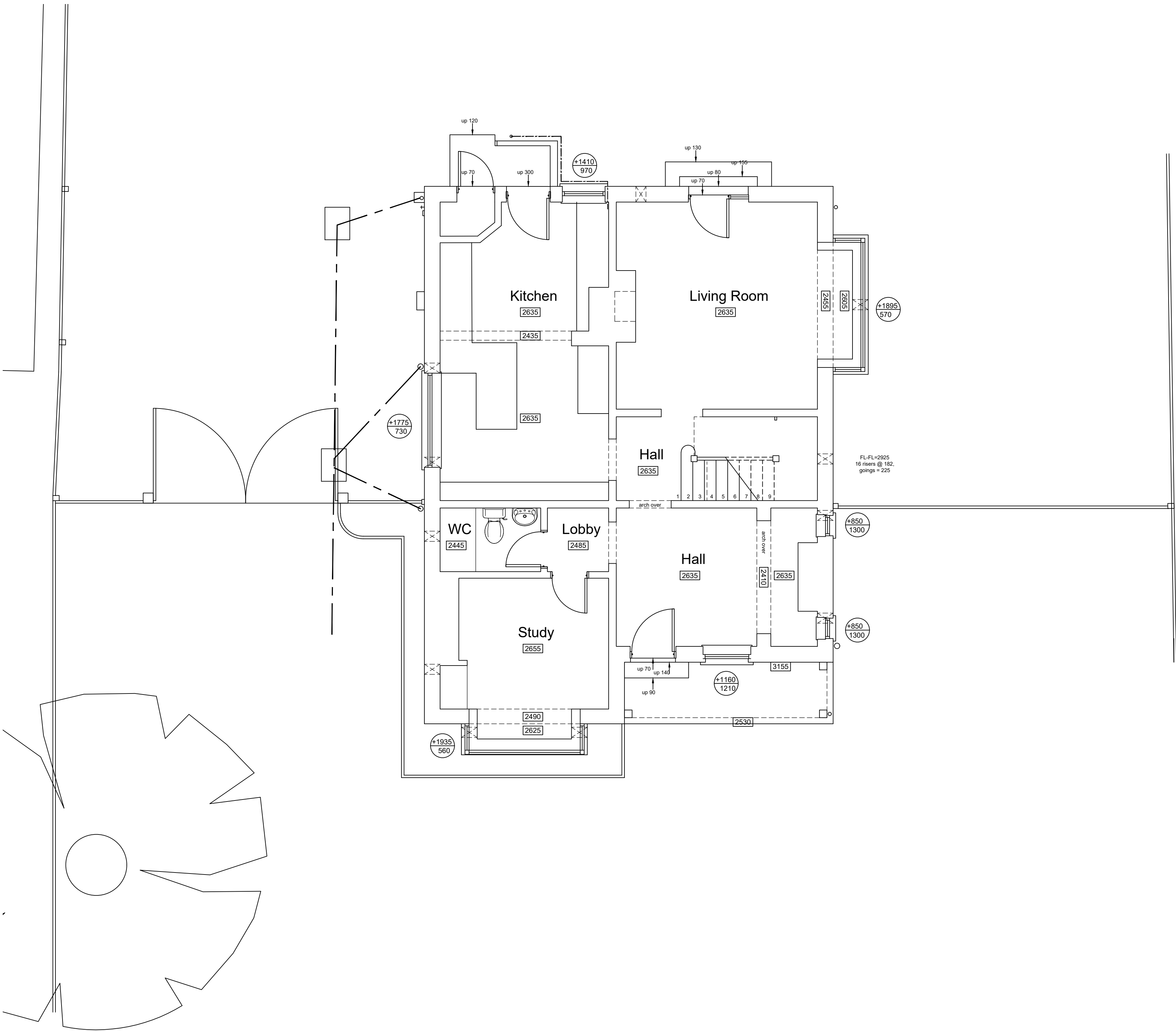
Ground Floor
