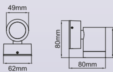
KSR1320
