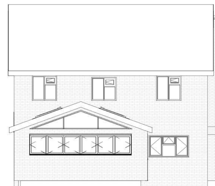
Proposed Elevation-Rear
