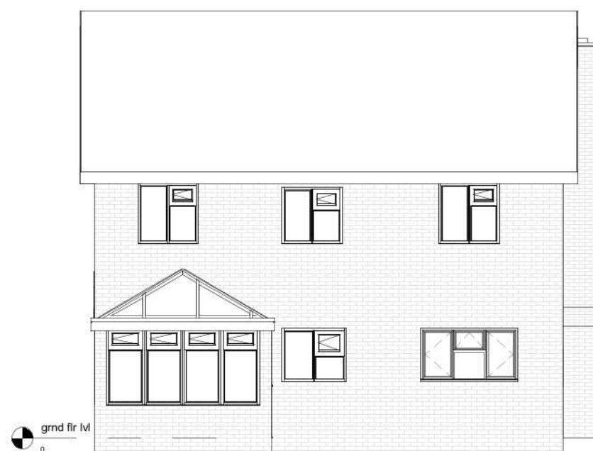
Existing Elevation-Rear
