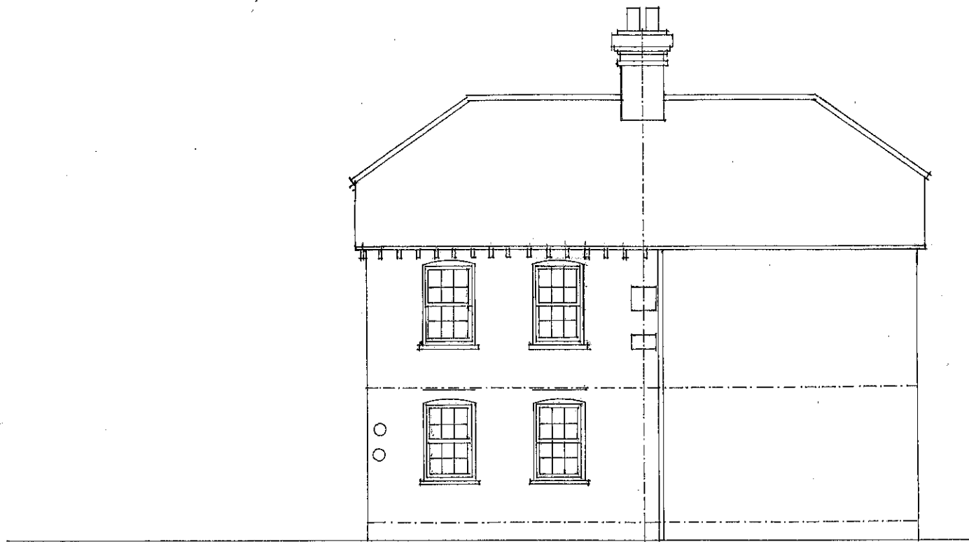
SOUTH WEST ELEVATION TO CLIMPING ST
