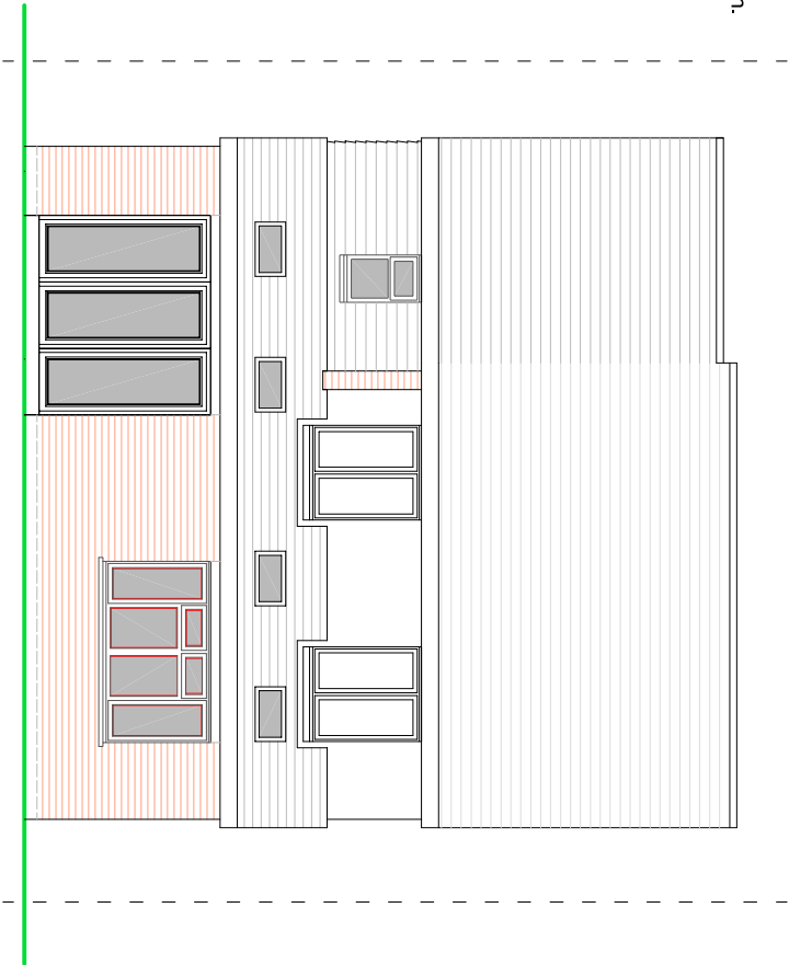
REAR ELEVATION
