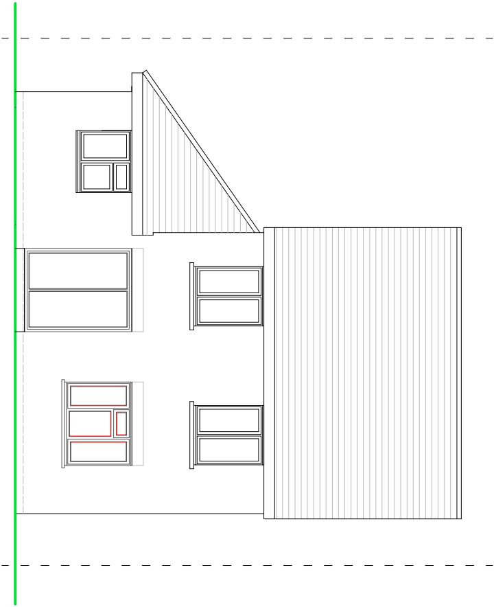
REAR ELEVATION
