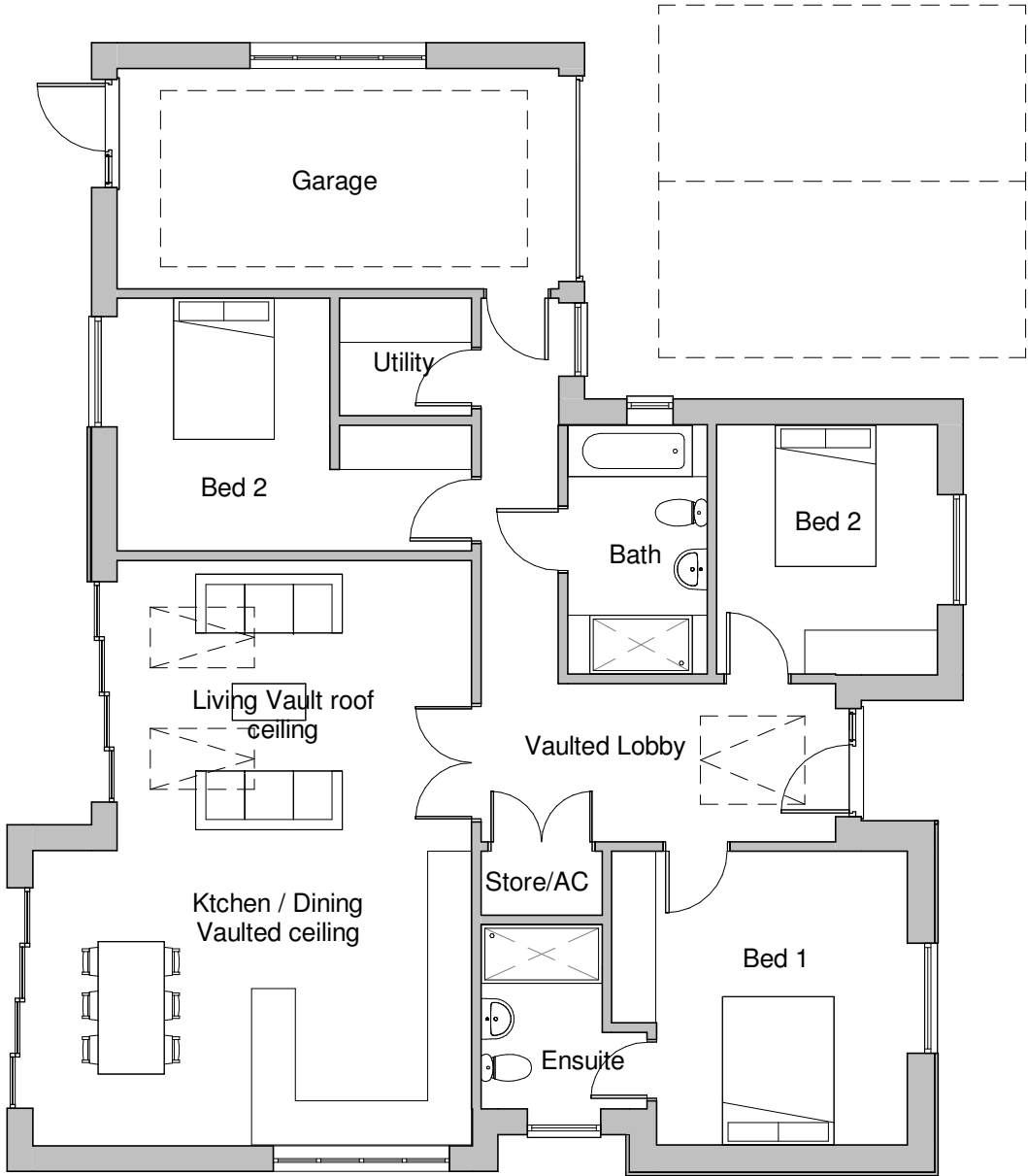
1 0 Ground Floor FFL 1 : 100
