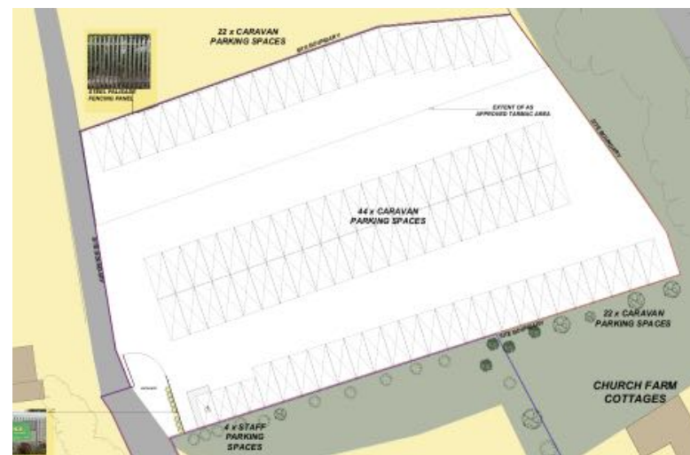
Figure 2: Site Layout (proposed)
