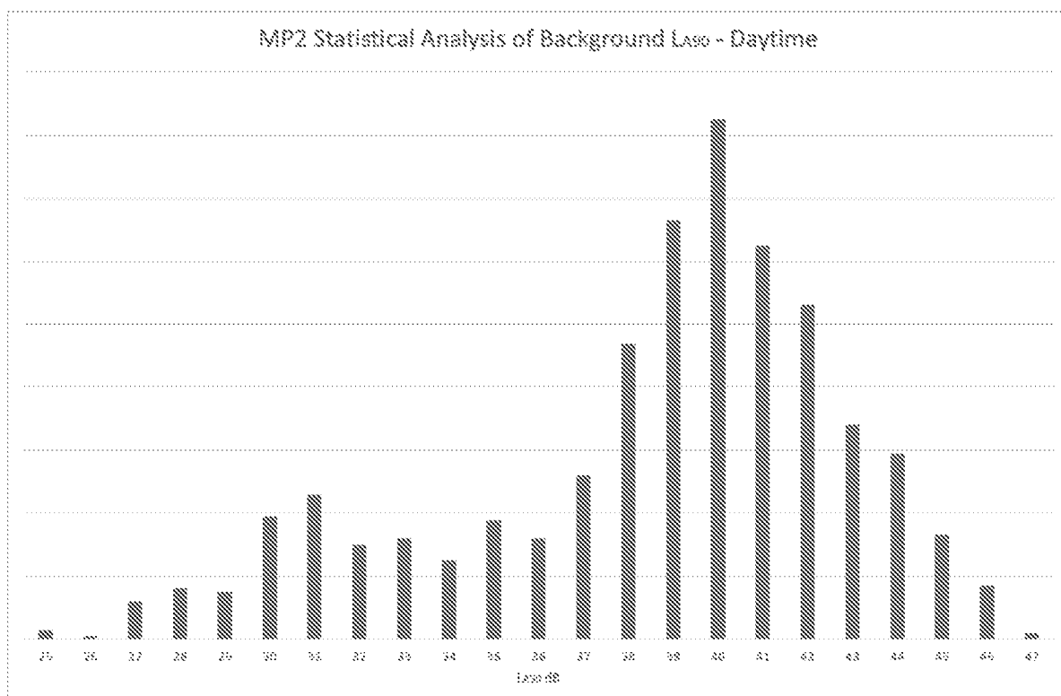
FIGURE 10: STATISTICAL ANALYSIS OF L_{A90} BACKGROUND – DAYTIME – MP2
