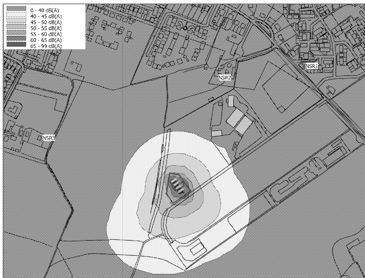
FIGURE 5: SPECIFIC SOUND LEVEL MAP
