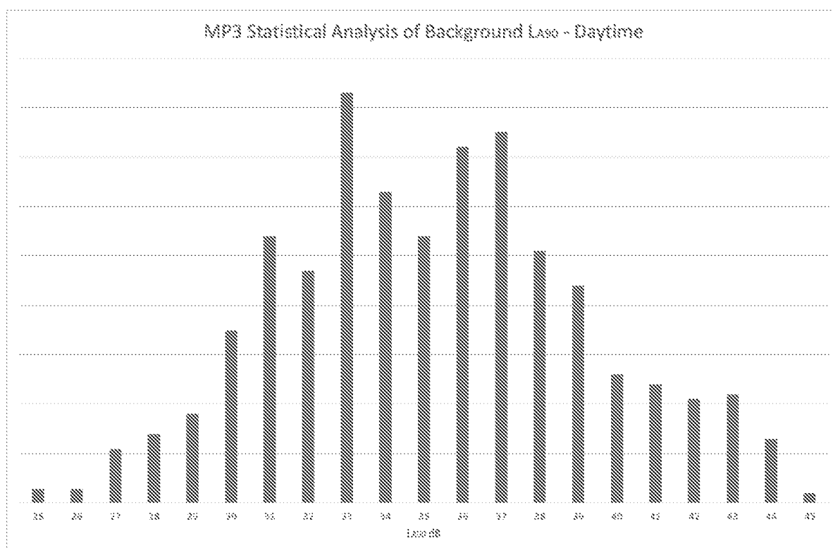
FIGURE 13: STATISTICAL ANALYSIS OF L_{A90} BACKGROUND – DAYTIME – MP3
