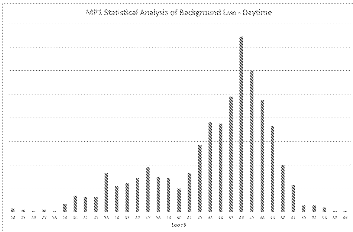
FIGURE 7: STATISTICAL ANALYSIS OF L_{A90} BACKGROUND – DAYTIME – MP1
