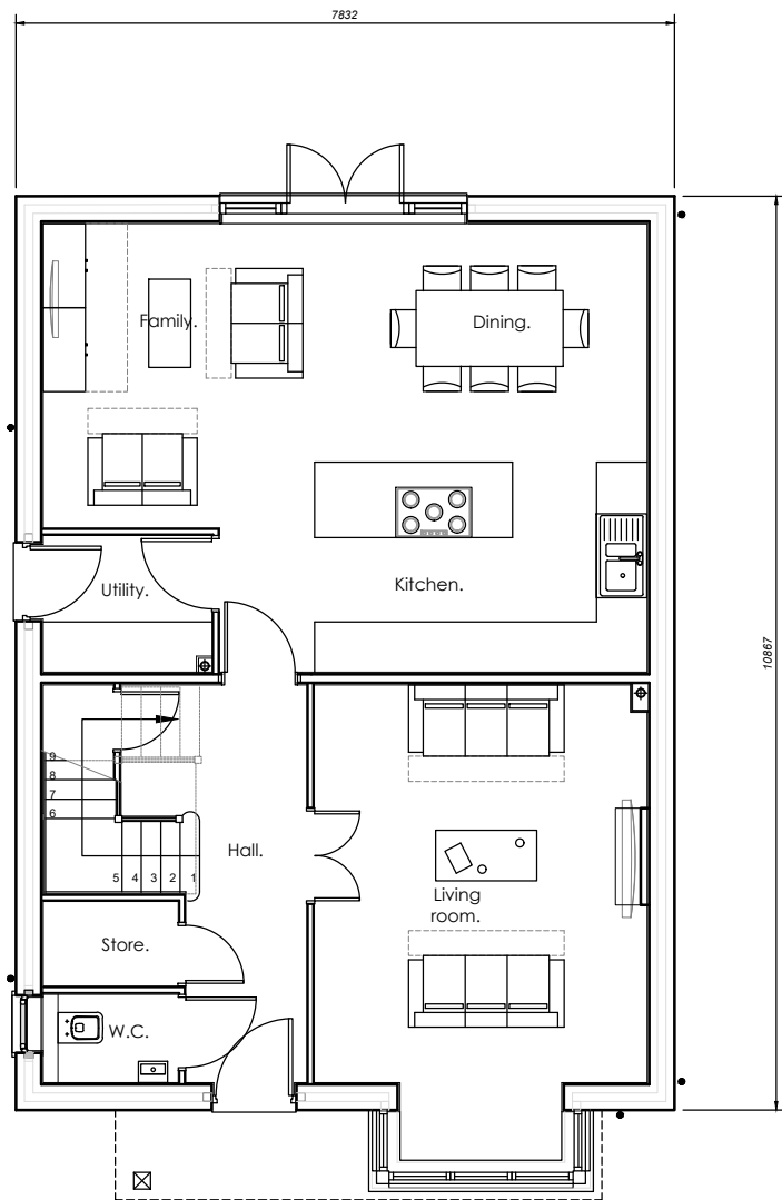
As Plots: 9 Handed Plots: Ground Floor Plan TYPE E 4b7p (Gross Internal)Floor Area = 1496sqft / 139m2
