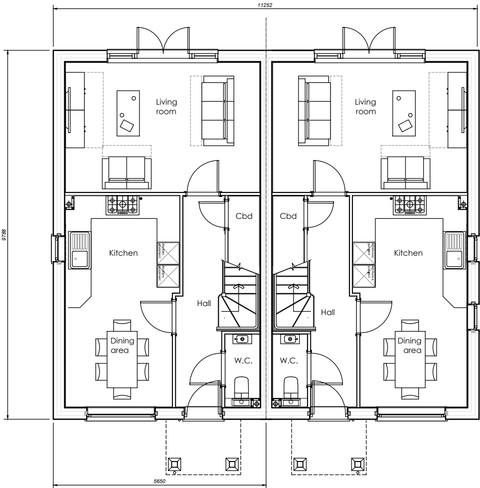
As Plots: 2 Handed Plots: 3 Ground Floor Plan TYPE B 3b5p (Gross Internal)Floor Area = 1002sqft / 93.1m2
