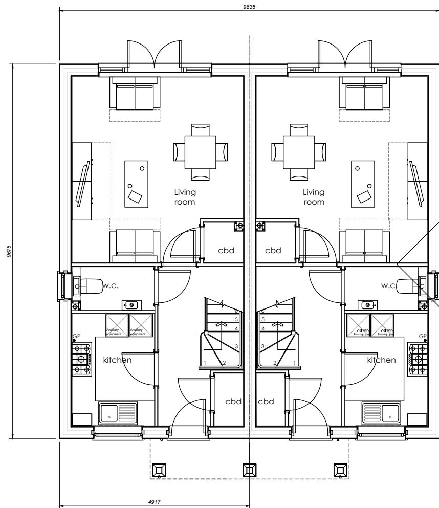
As Plots: 4 Handed Plots: 5 Ground Floor Plan TYPE C 2b4p (Gross Internal)Floor Area = 857sqft / 79.7m2
