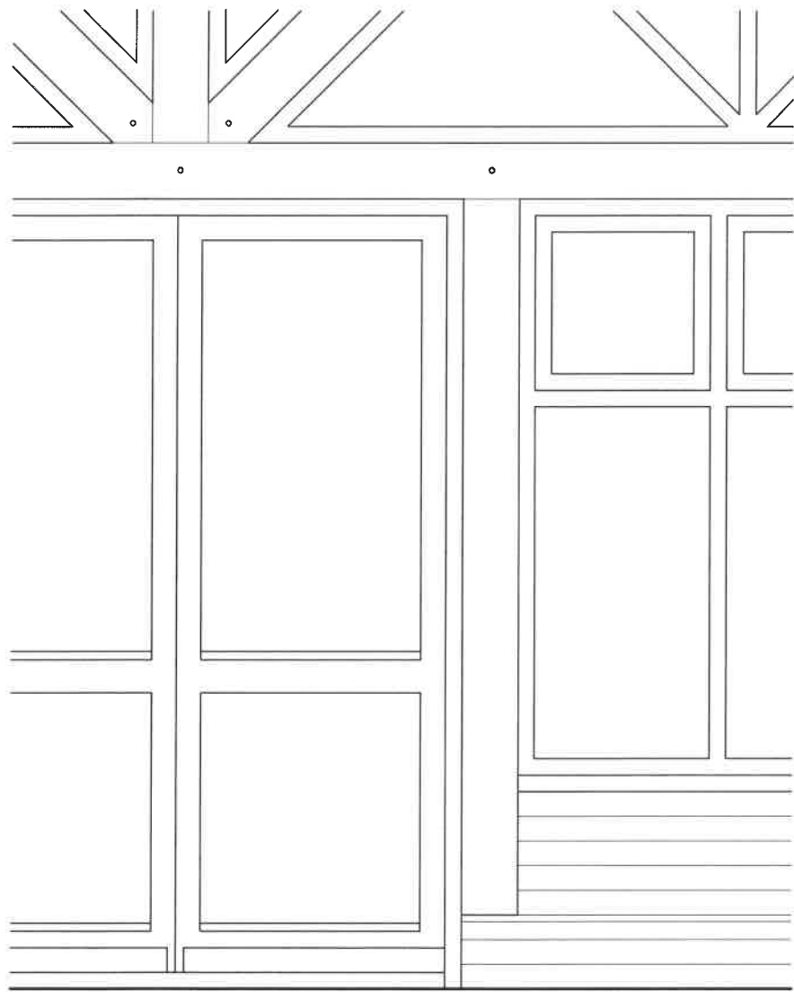
Proposed Glazed Screen Part Elevation @ 1:20
