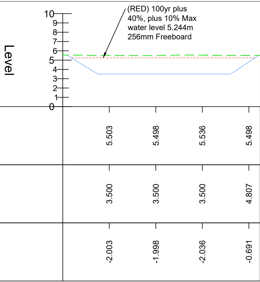
ALIGNMENT - BASIN 1 A-A - LONGSECTION SCALE: H 1:500,V 1:250. DATUM: 0.000
