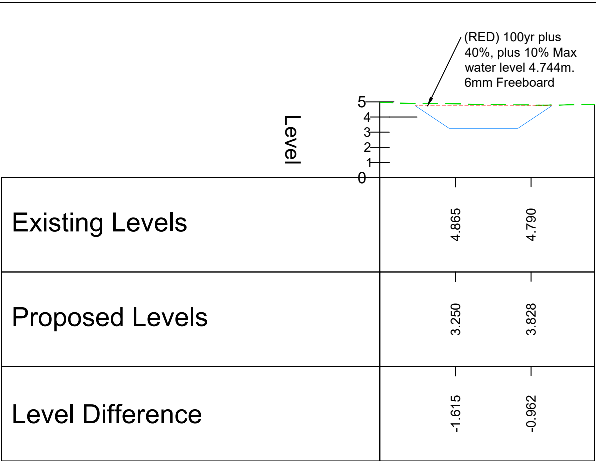
ALIGNMENT - BASIN 6 A-A - LONGSECTION SCALE: H 1:500,V 1:250. DATUM: 0.000
