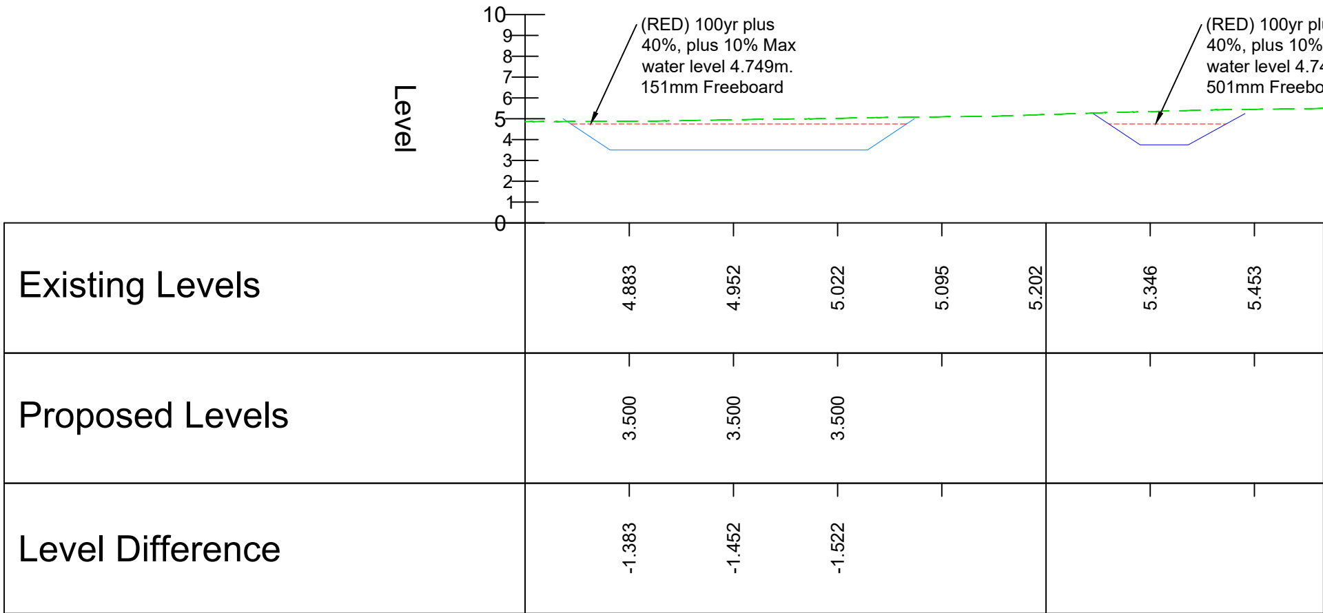
ALIGNMENT - BASIN 7&8 B-B - LONGSECTION SCALE: H 1:500,V 1:250. DATUM: 0.000
