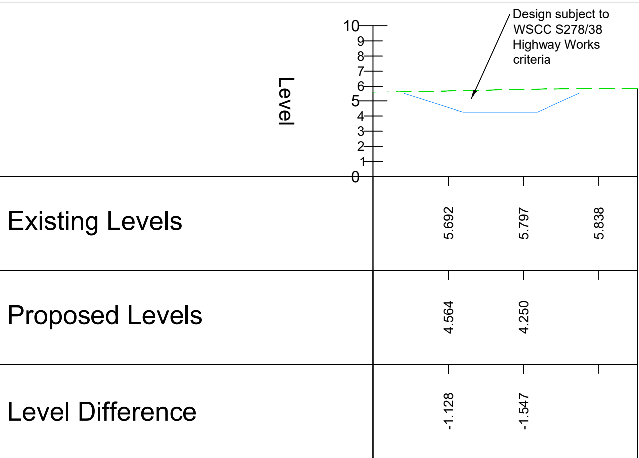
ALIGNMENT - BASIN S278 A-A - LONGSECTION SCALE: H 1:500,V 1:250. DATUM: 0.000
