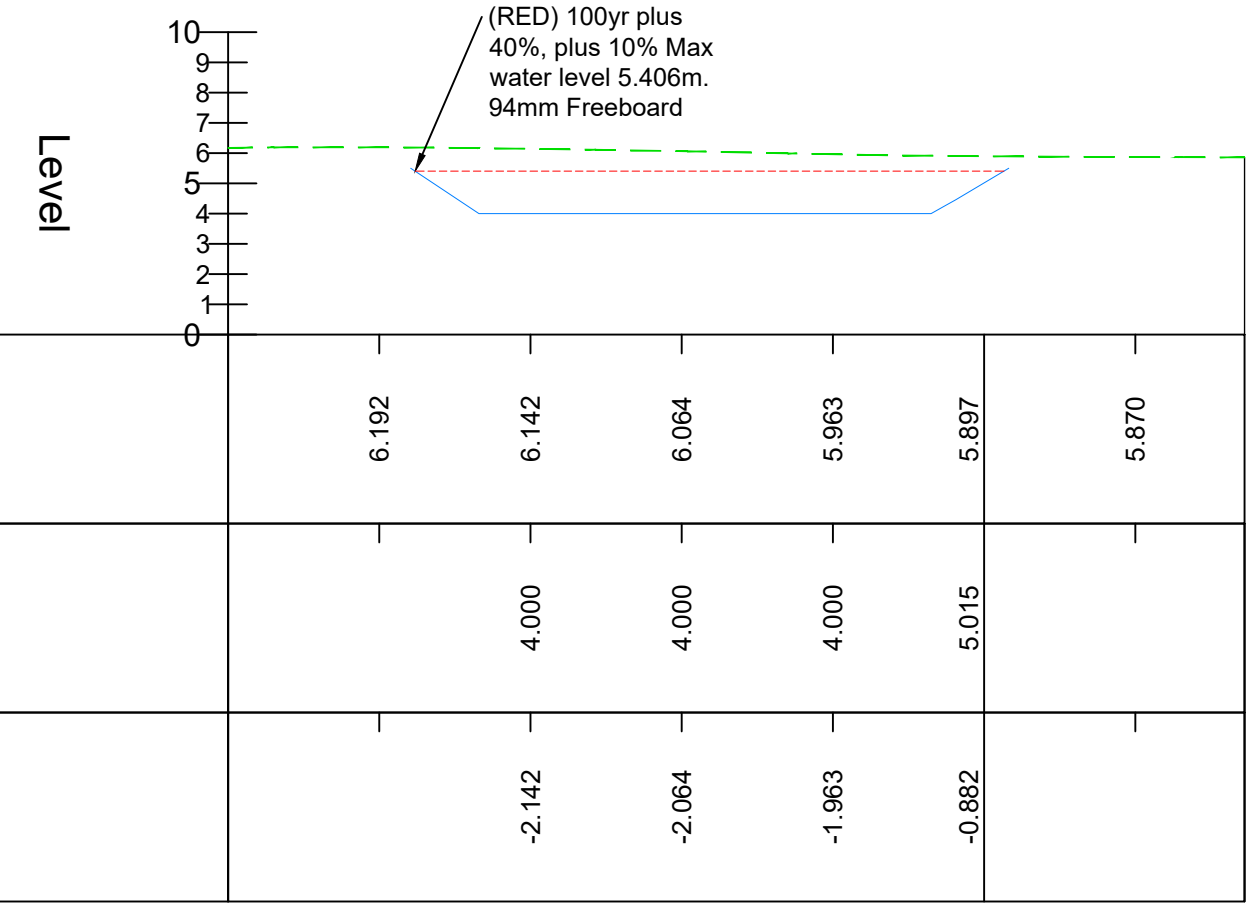
ALIGNMENT - BASIN 2 B-B - LONGSECTION SCALE: H 1:500,V 1:250. DATUM: 0.000
