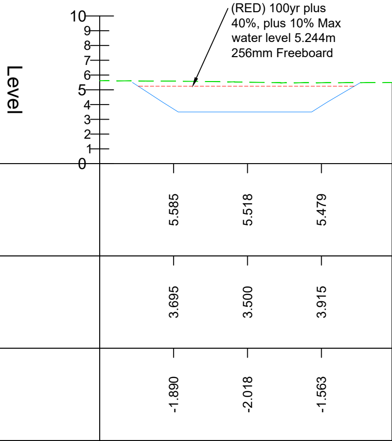
ALIGNMENT - BASIN 1 B-B - LONGSECTION SCALE: H 1:500,V 1:250. DATUM: 0.000
