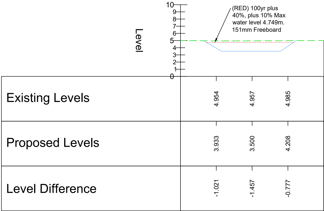
ALIGNMENT - BASIN 7 A-A - LONGSECTION SCALE: H 1:500,V 1:250. DATUM: 0.000
