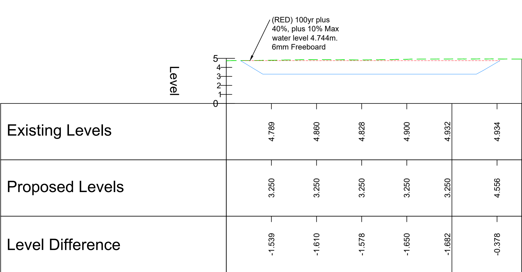
ALIGNMENT - BASIN 6 B-B - LONGSECTION SCALE: H 1:500,V 1:250. DATUM: 0.000
