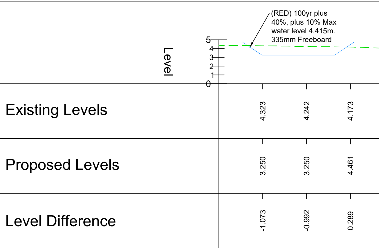
ALIGNMENT - BASIN 4 A-A - LONGSECTION SCALE: H 1:500,V 1:250. DATUM: 0.000
