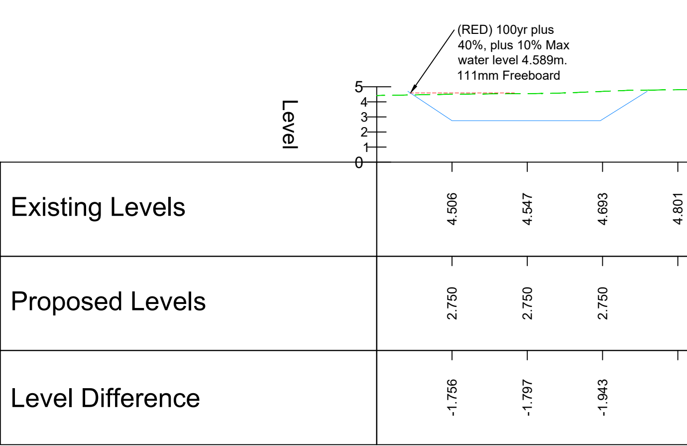
ALIGNMENT - BASIN 5 B-B - LONGSECTION SCALE: H 1:500,V 1:250. DATUM: 0.000
