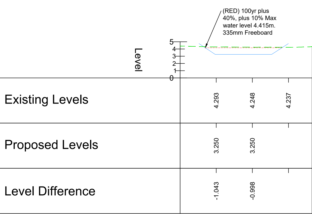
ALIGNMENT - BASIN 4 B-B - LONGSECTION SCALE: H 1:500,V 1:250. DATUM: 0.000
