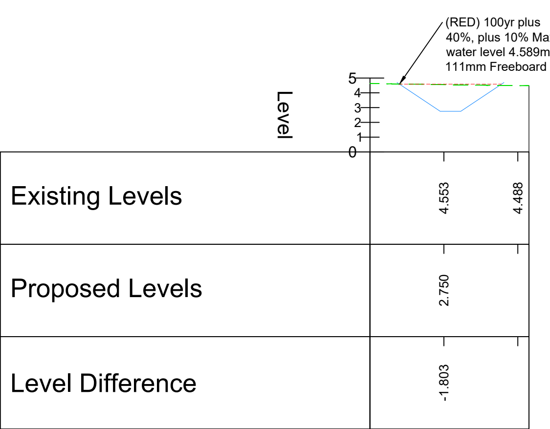
ALIGNMENT - BASIN 5 A-A - LONGSECTION SCALE: H 1:500,V 1:250. DATUM: 0.000
