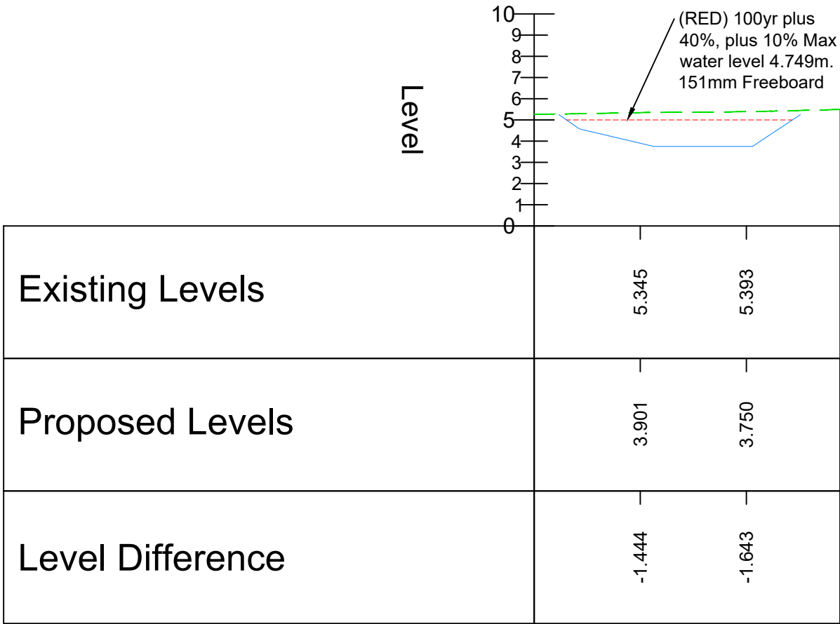
ALIGNMENT - BASIN 8 A-A - LONGSECTION SCALE: H 1:500,V 1:250. DATUM: 0.000
