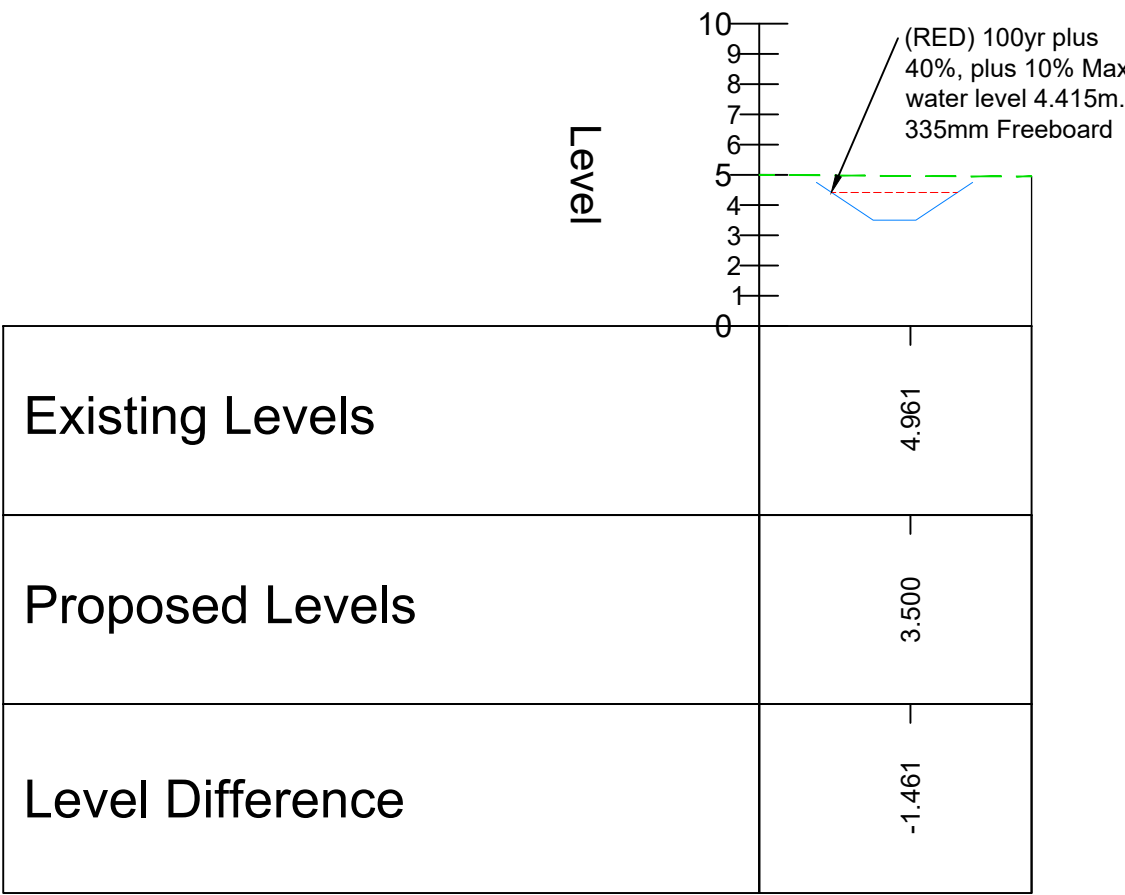
ALIGNMENT - BASIN 3 B-B - LONGSECTION SCALE: H 1:500,V 1:250. DATUM: 0.000
