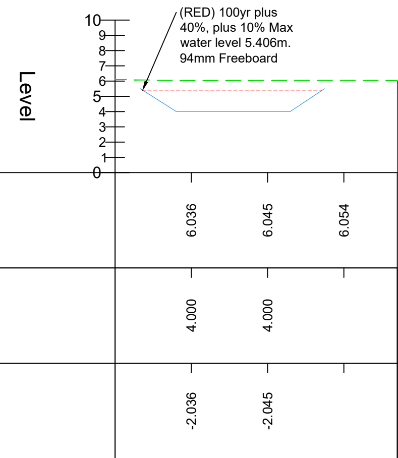
ALIGNMENT - BASIN 2 A-A - LONGSECTION SCALE: H 1:500,V 1:250. DATUM: 0.000
