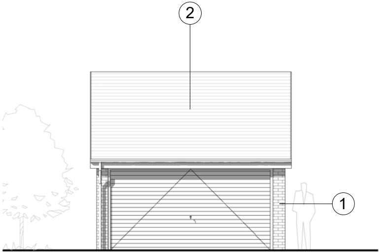
Front Elevation 1 : 100
