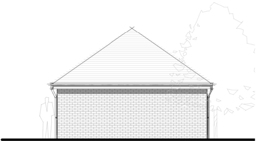
Rear Elevation 1 : 100
