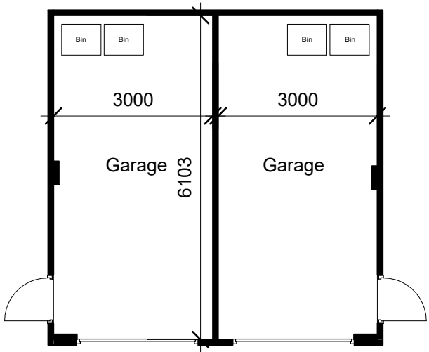
Level 00-Ground Floor 1 : 100
