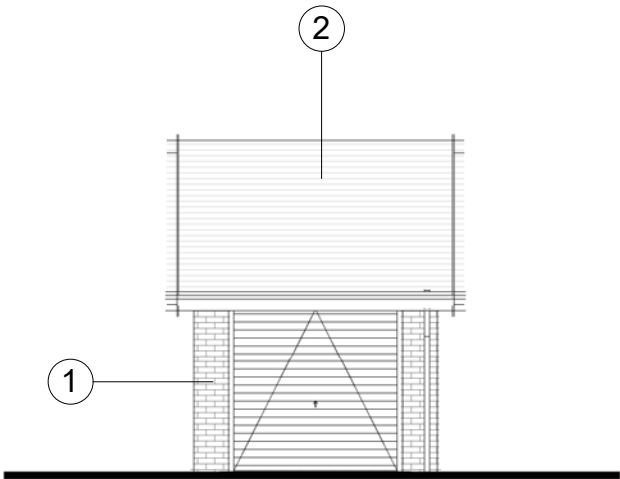
Front Elevation 1 : 100
