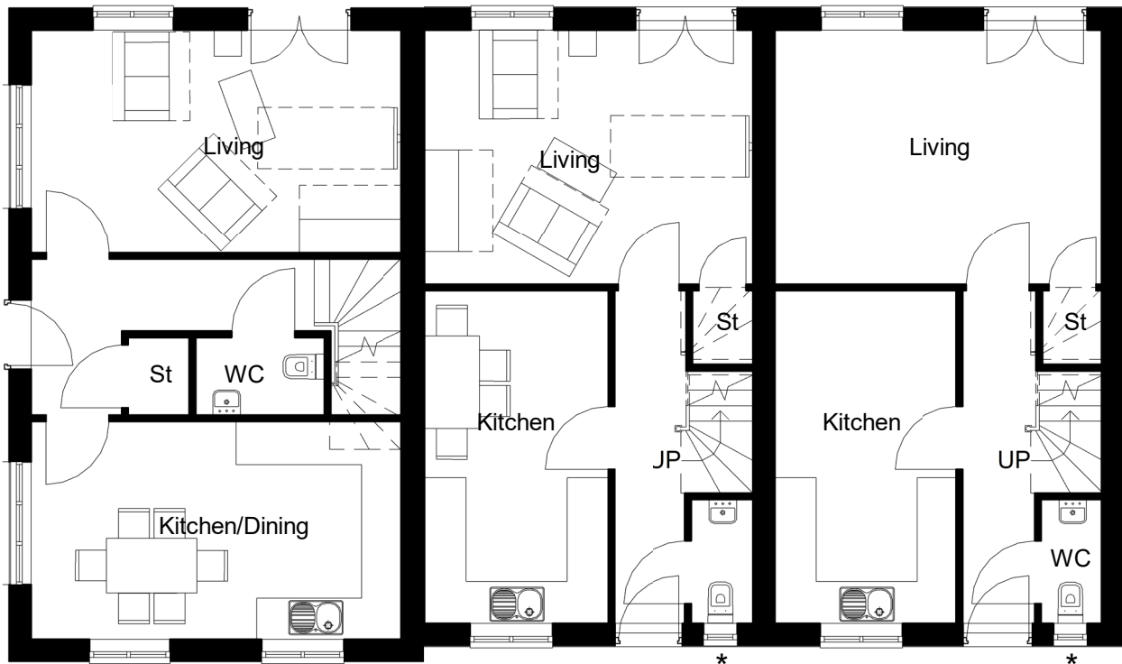
Level 00-Ground Floor 1 : 100
