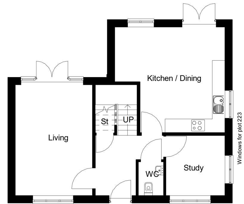
Level 00-Ground Floor 1 : 100
