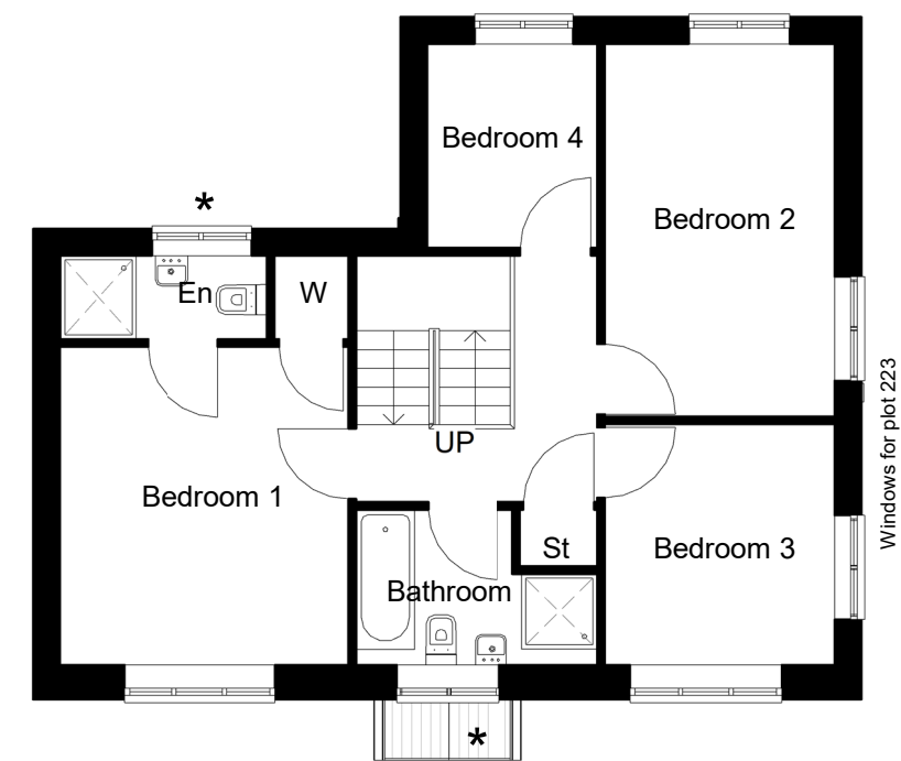
Level 01-First Floor 1 : 100
