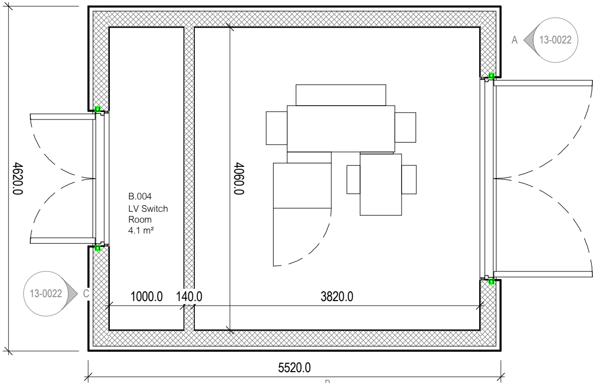
01 Substation Floor Plan 1 : 50
