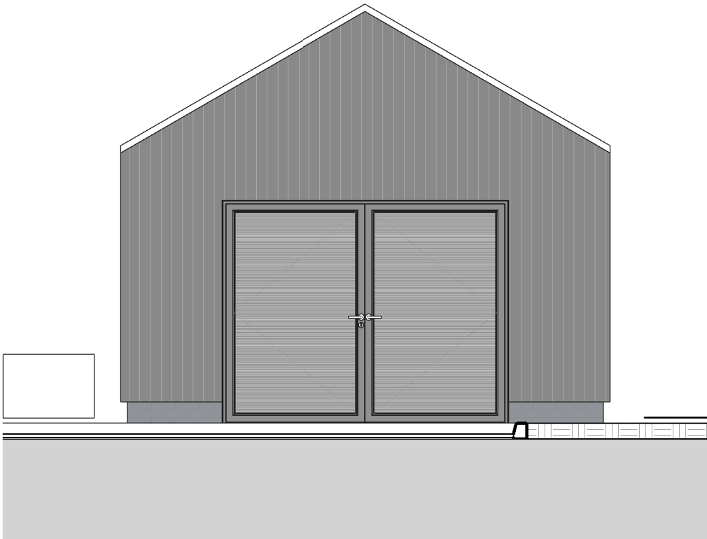
A Substation Elevation A 1 : 50
