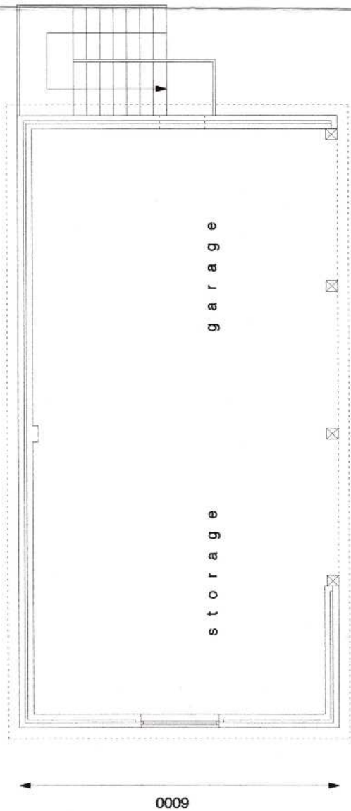
Proposed Ground Floor Plan at 1: 100 scale
