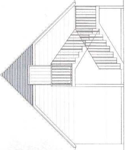
6000 Proposed Side Elevation at 1: 100 scale
