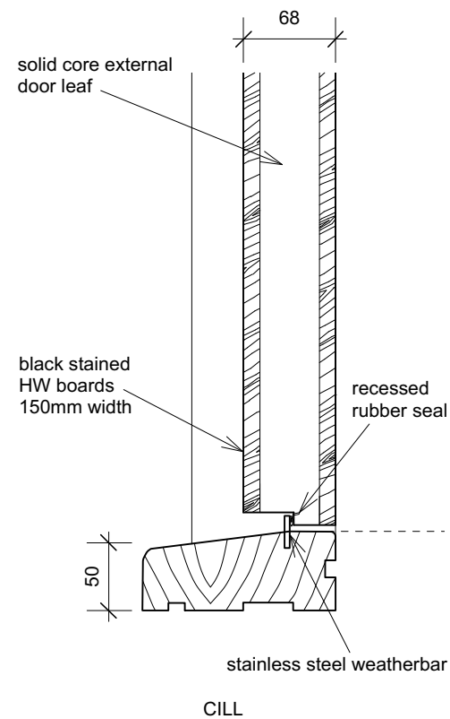
Detail D4 External Entrance Doors
