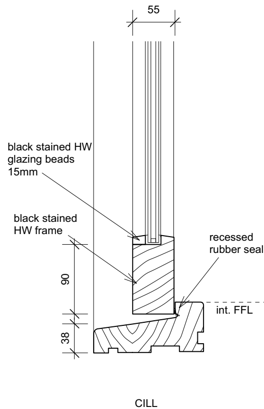
Detail D3 Patio Doors
