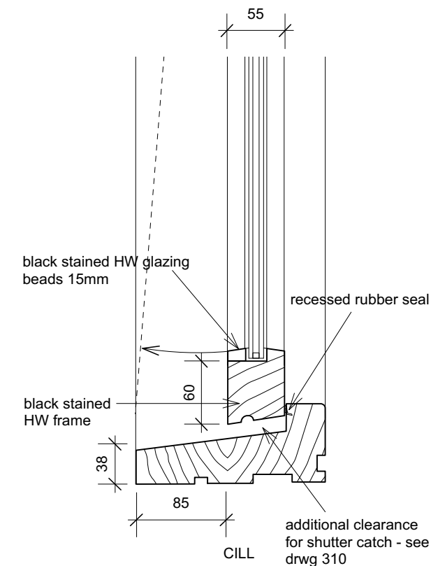
Detail D1 Hardwood Casement Window
