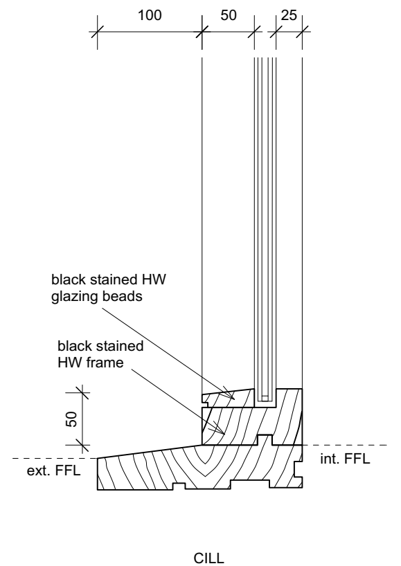
Detail D5 Fixed Windows
