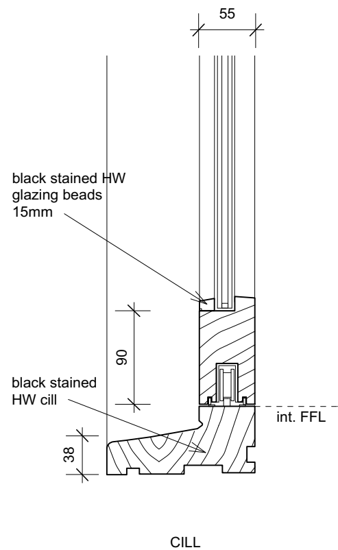
Detail D2 Sliding Doors
