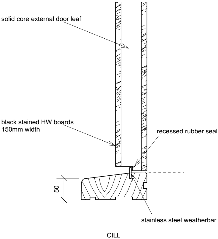
Detail D4 External Entrance Doors
