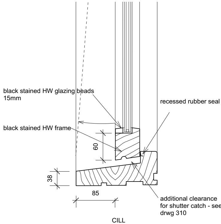
Detail D1 Hardwood Casement Window
