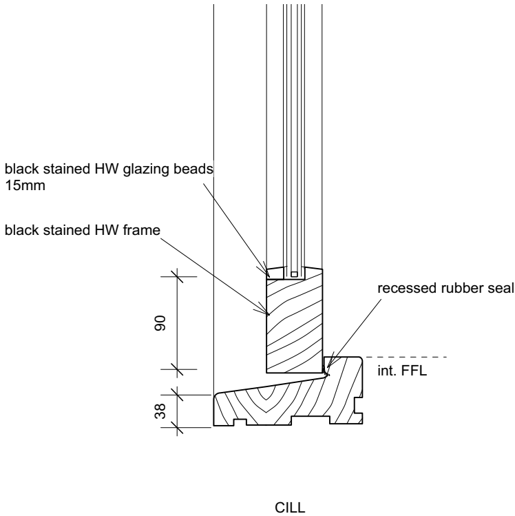
Detail D3 Patio Doors
