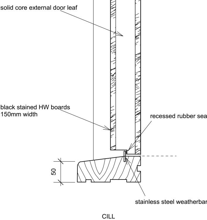
Detail D4 External Entrance Doors
