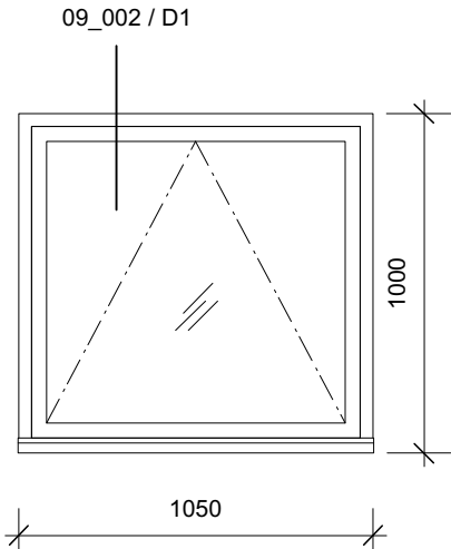
WG02 FINISH: Hardwood Top hung GLAZING: Black stained HW IRONMONGERY 24mm DGUs, Argon filled All bronze: external hinges or sliding stays, handle, recessed window lock, opening stay
