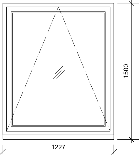
WG03 FINISH: Hardwood Top hung (Original window opening) GLAZING: Black stained HW IRONMONGERY 24mm DGUs, Argon filled All bronze: external hinges or sliding stays, handle, recessed window lock, opening stay
