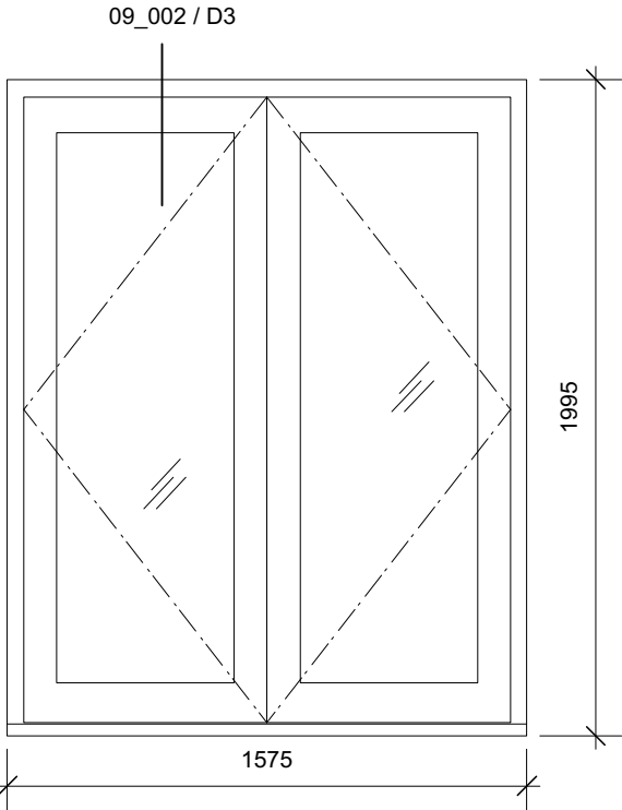
WG01 FINISH: Hardwood Patio Doors GLAZING: Black Stained HW IRONMONGERY 24mm DGUs, Argon filled Bronze external hinges, bronze lever handle, Mortice latchlock, Mortice deadlock with thumbturn Recessed flushbolt top+bottom to slave leaf
