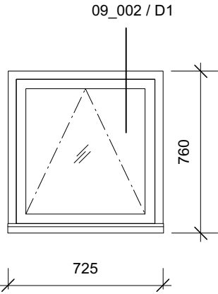
WG08 FINISH: Hardwood Top hung GLAZING: Black stained HW IRONMONGERY 24mm DGUs, Argon filled All bronze: external hinges or sliding stays, handle, recessed window lock, opening stay
