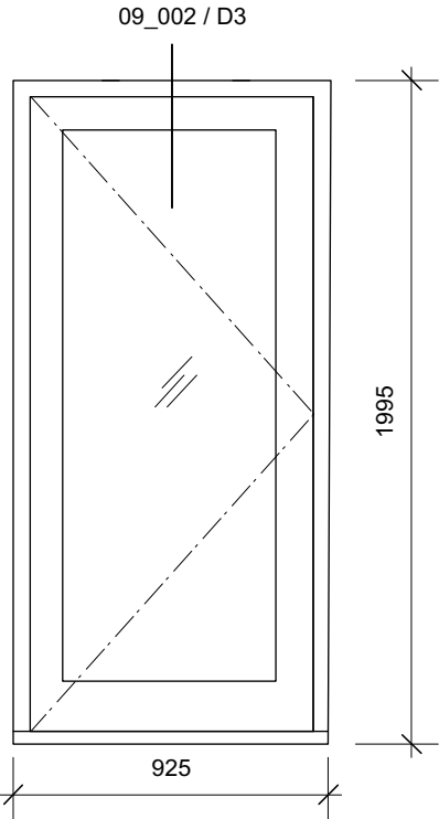
WG05 FINISH: Hardwood Patio Door GLAZING: Black stained HW IRONMONGERY 24mm DGUs, Argon filled Bronze external hinges, bronze lever handle, Mortice latchlock, Mortice deadlock with thumbturn
