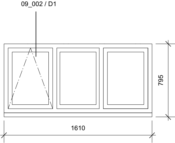
WG04 FINISH: Hardwood Top hung and fixed GLAZING: Black stained HW IRONMONGERY 24mm DGUs, Argon filled All bronze: external hinges or sliding stays, handle, recessed window lock, opening stay
