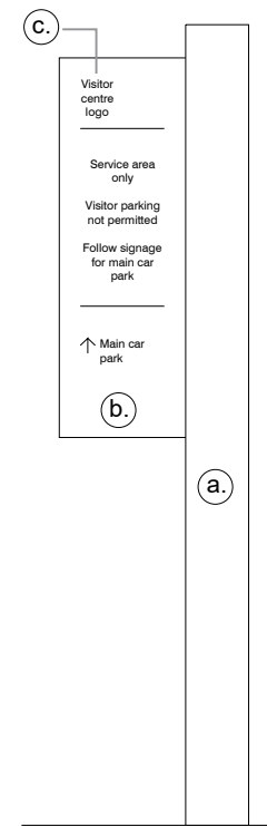
8. SERVICE AREA SIGNAGE 1:20
