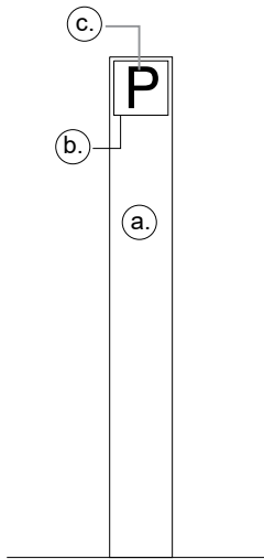
3. ACCESSIBLE PARKING SIGNAGE 1:20
