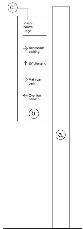
1. PARKING WAY-FINDING SIGNAGE 1:20
