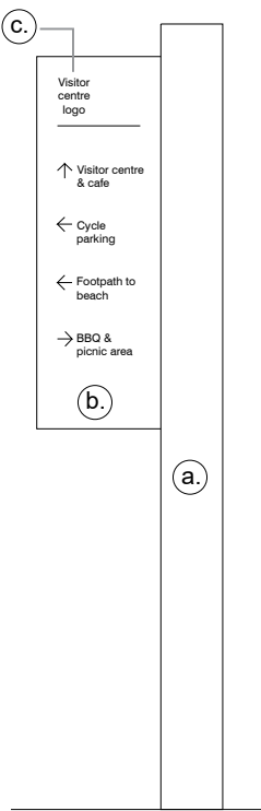
2. VISITOR CENTRE WAY-FINDING SIGNAGE 1:20
