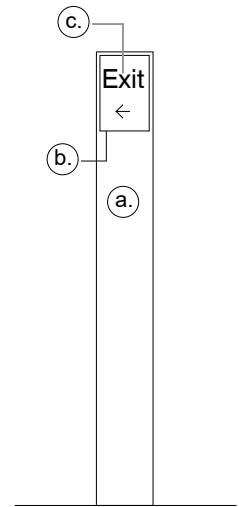
7. EXIT SIGNAGE 1:20
