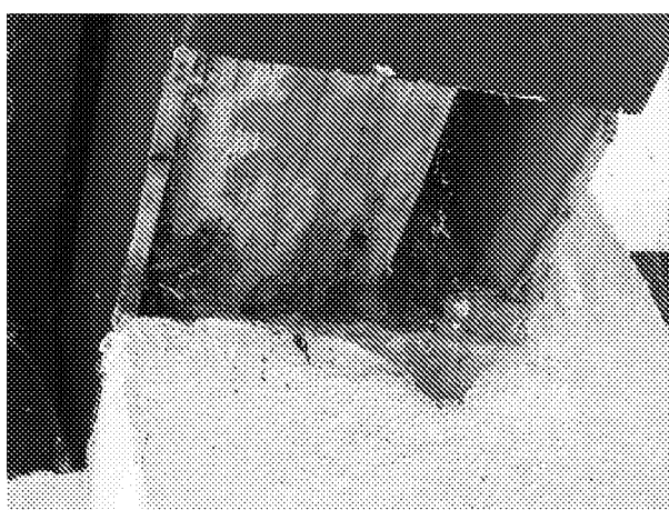
DSC02874 Rotted bearing end to timber beam
