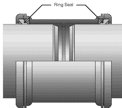
Figure 10: Ring Seal jointing
