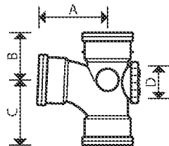
D/S Equal Access Junction - 87.5°
