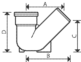
S/S Universal Gully Trap
