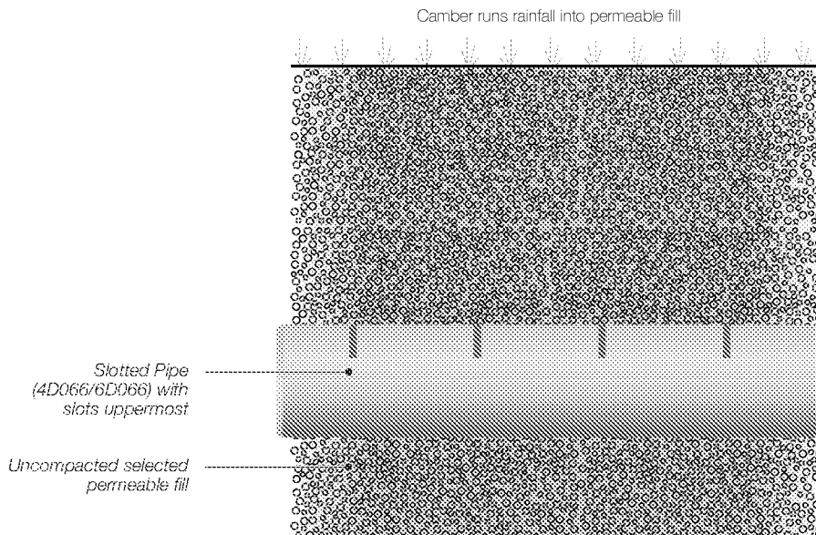
Figure 37: French Drain
