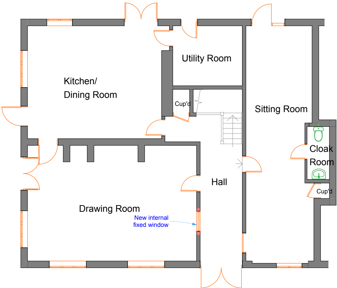
Ground Floor - Proposed
