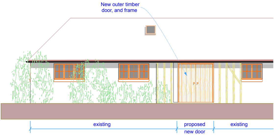
North Elevation outer door closed
