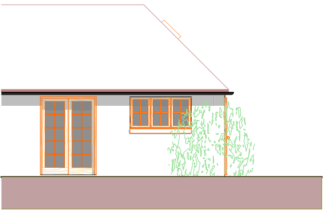
East Elevation
