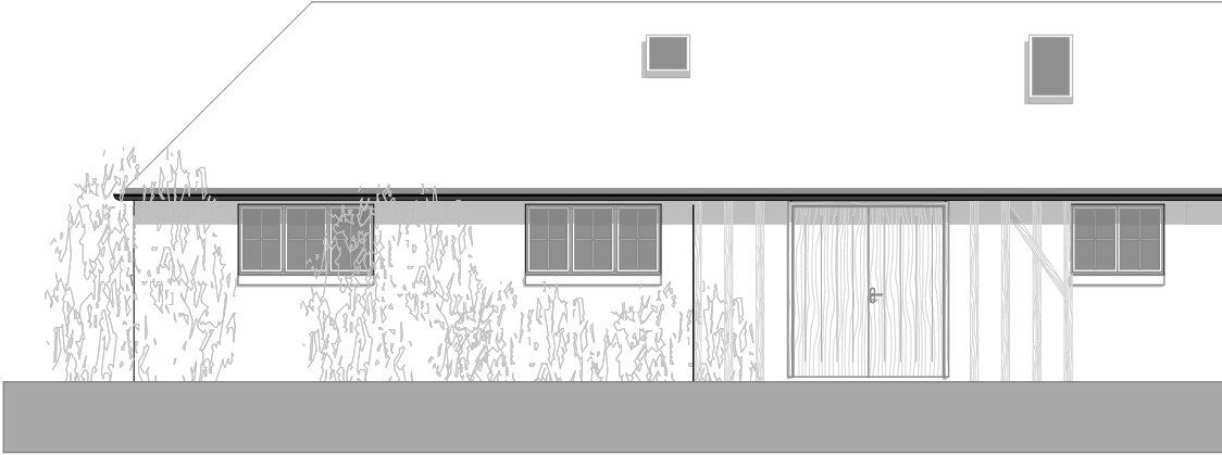
North Elevation
