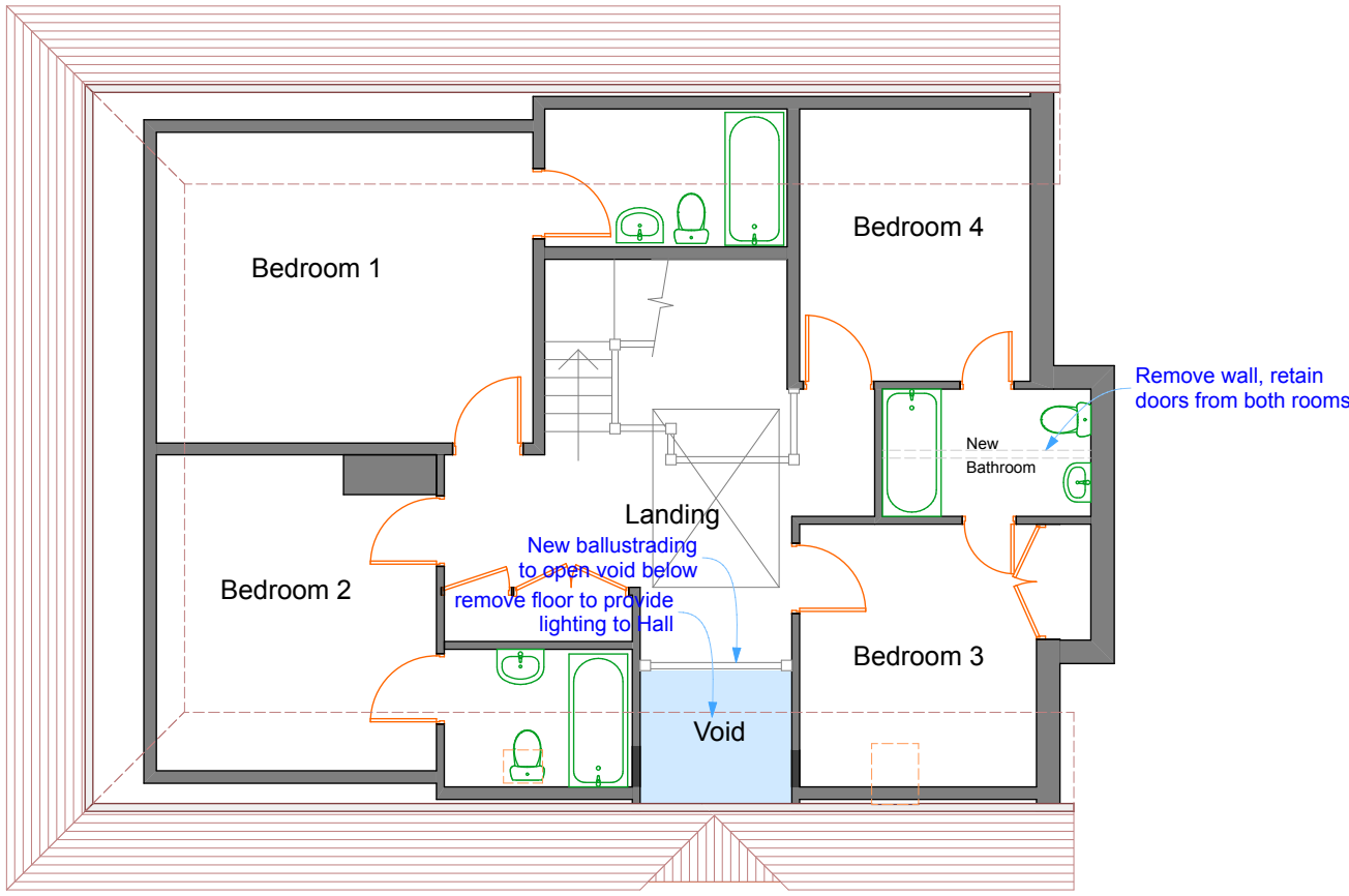
First Floor
