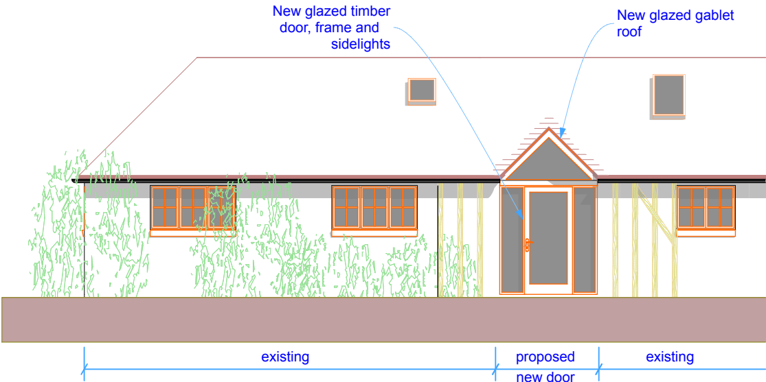
North Elevation
