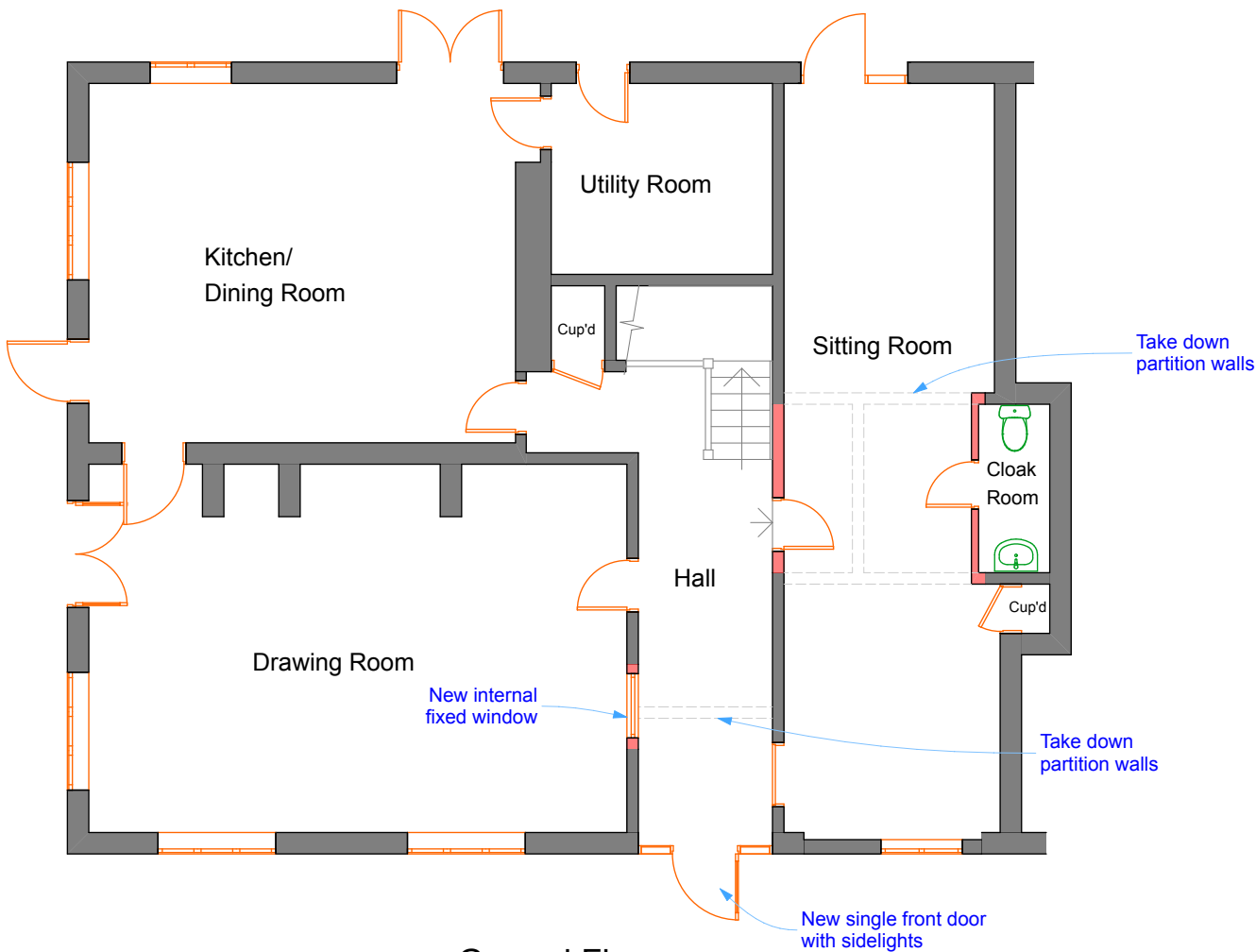
Ground Floor
