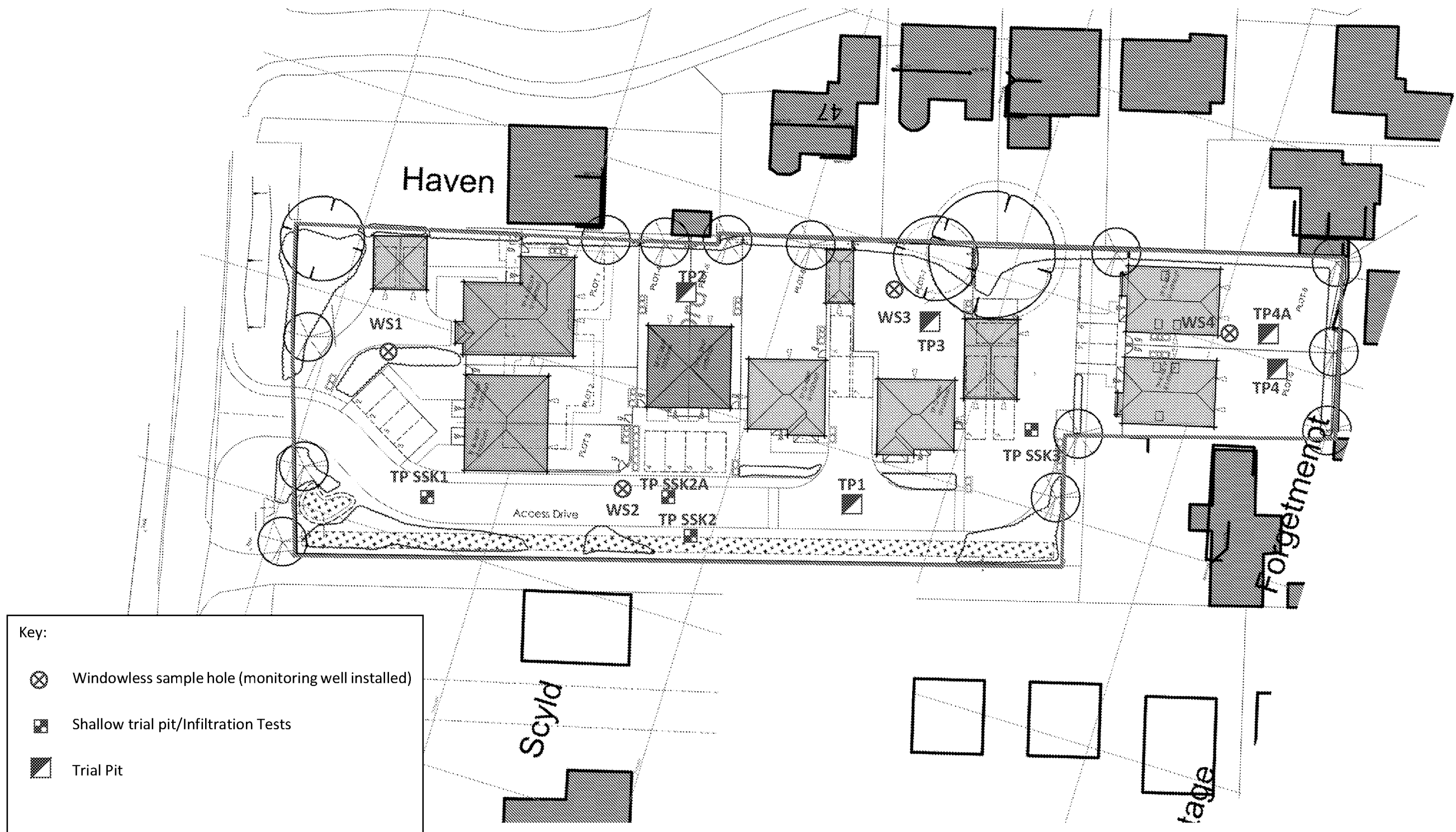
EXPLORATORY HOLE LOCATION PLAN
