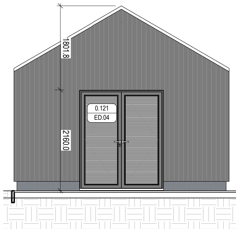
C Substation Elevation C 1 : 50
